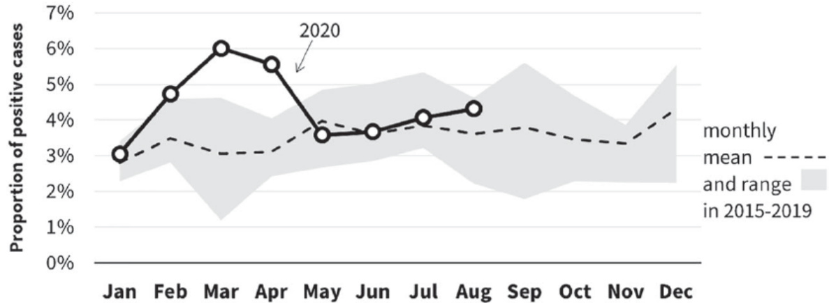
(b) Amphetamine
