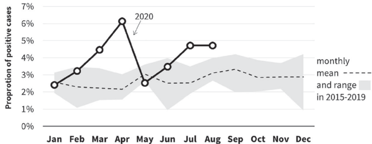
(b) Amphetamine
