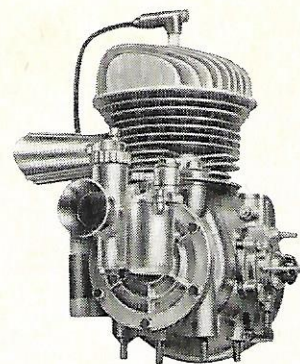
SAETTA V 16 Sport
