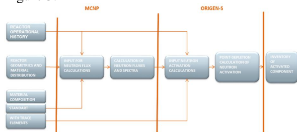
Figure 3: Calculation scheme.
